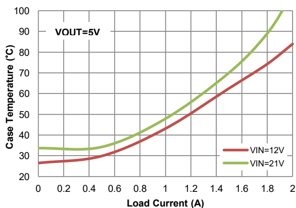
Figure 10. Case Temperature vs. Load Current
