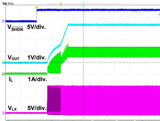
1ms/div. Figure 20. Power On through \overline{SHDN} Waveform
