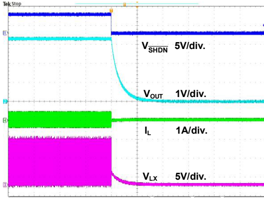
10ms/div. Figure 21. Power Off through \overline{SHDN} Waveform
