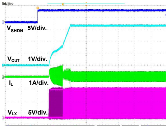
1ms/div. Figure 19. Power On through \overline{SHDN} Waveform
