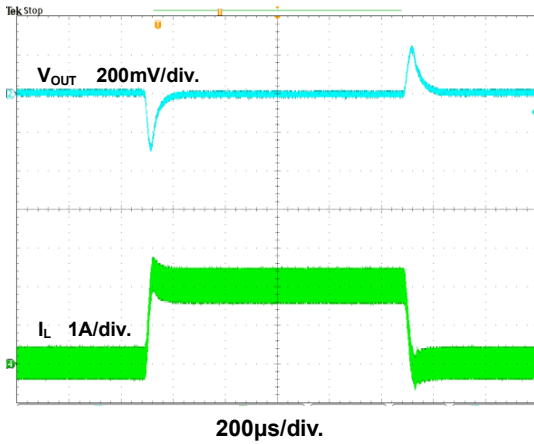
Figure 23. Load Transient Waveform
