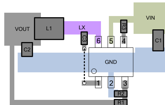
Figure 25. FR9801 Recommended Layout Diagram
