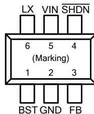
Figure 1. Pin Assignment of FR9801
