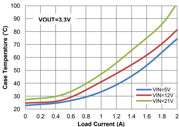
Figure 9. Case Temperature vs. Load Current
