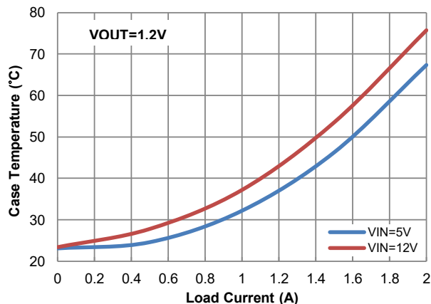
Figure 8. Case Temperature vs. Load Current
