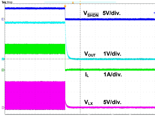
1ms/div. Figure 22. Power Off through \overline{SHDN} Waveform
