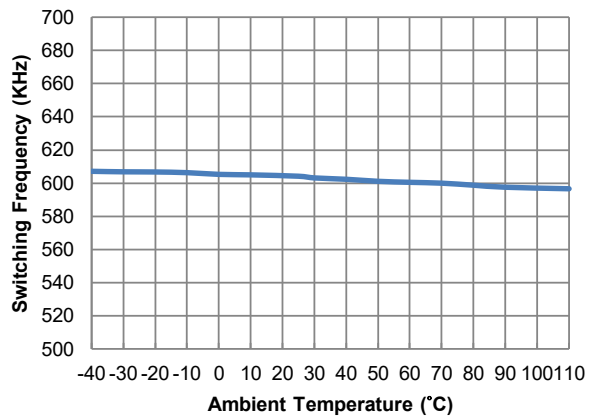
Figure 12. Switching Frequency vs. Temperature
