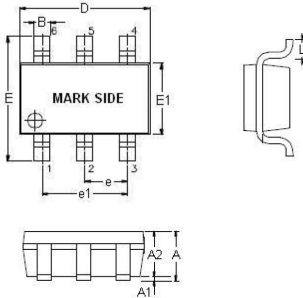
SOT-23-6 Package (Unit: mm)
