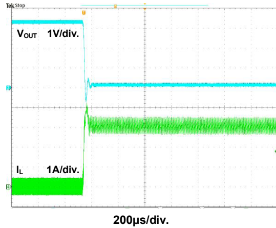
Figure 24. Short Circuit Test
