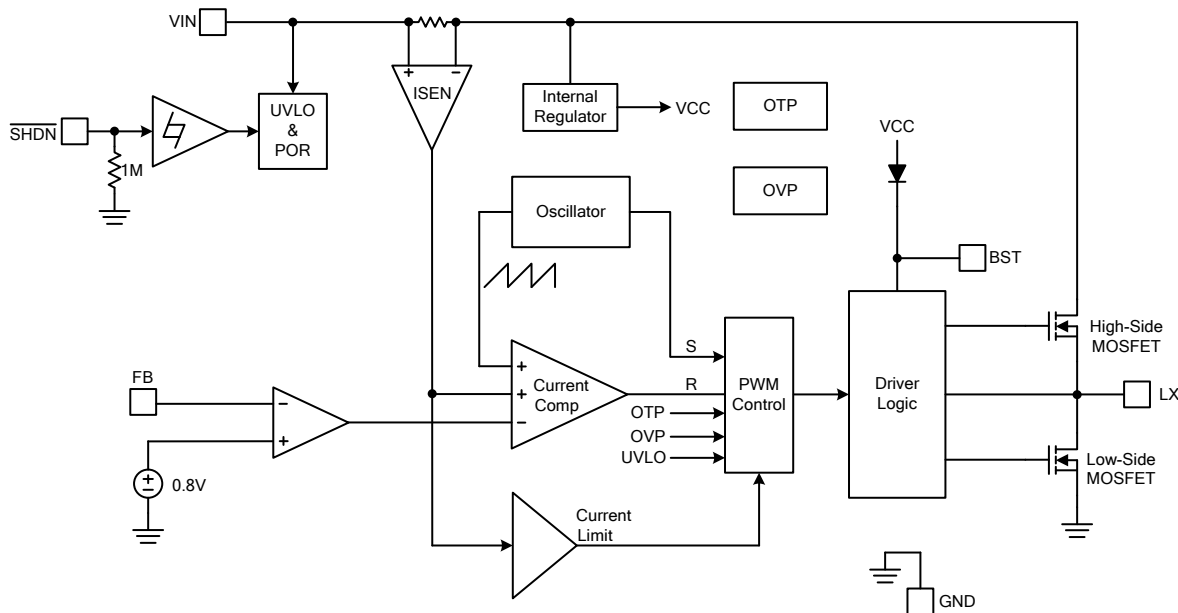
Figure 4. Block Diagram of FR9801
