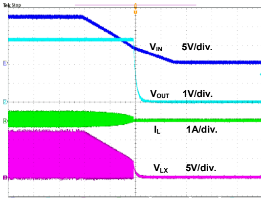
20ms/div. Figure 17. Power Off through VIN Waveform
