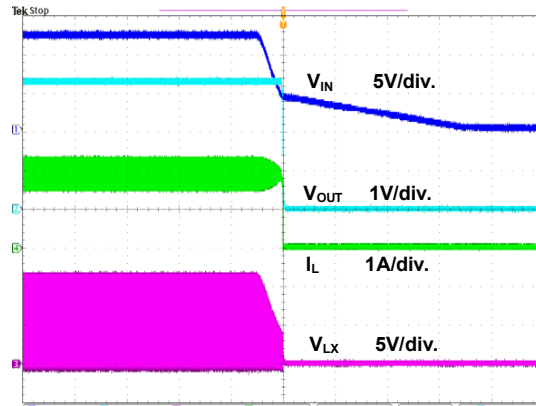
10ms/div. Figure 18. Power Off through VIN Waveform
